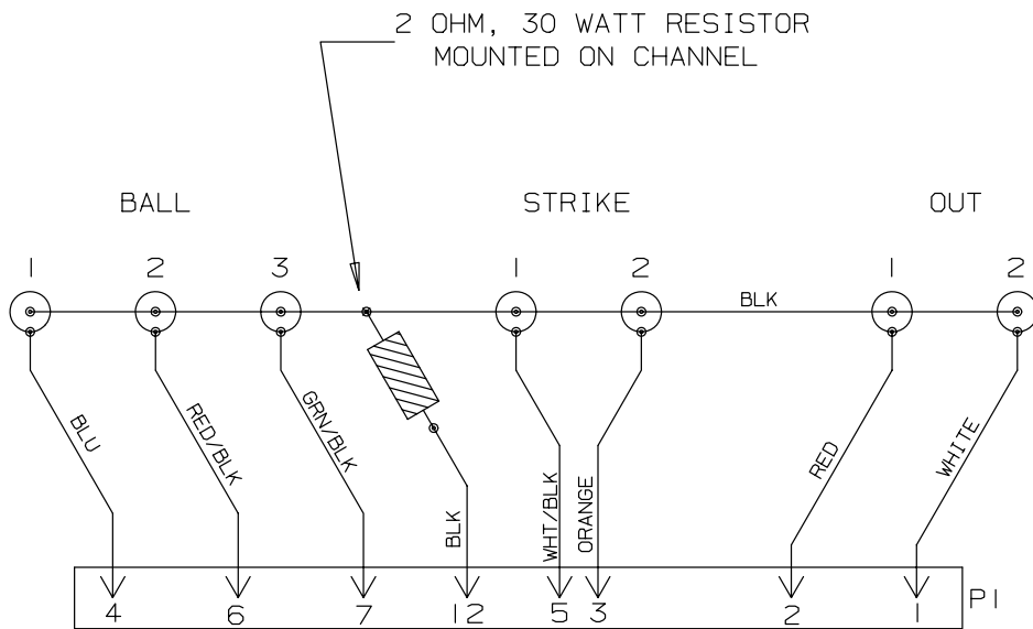
BALL, STRIKE, AND OUT WIRING
